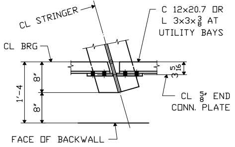
DETAIL B TYP LAP POSITION AT SOUTH ABUT.
